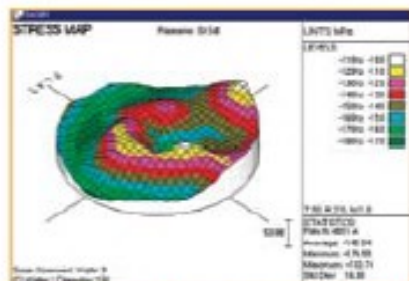
3D contour maps help monitor film stress uniformity.
